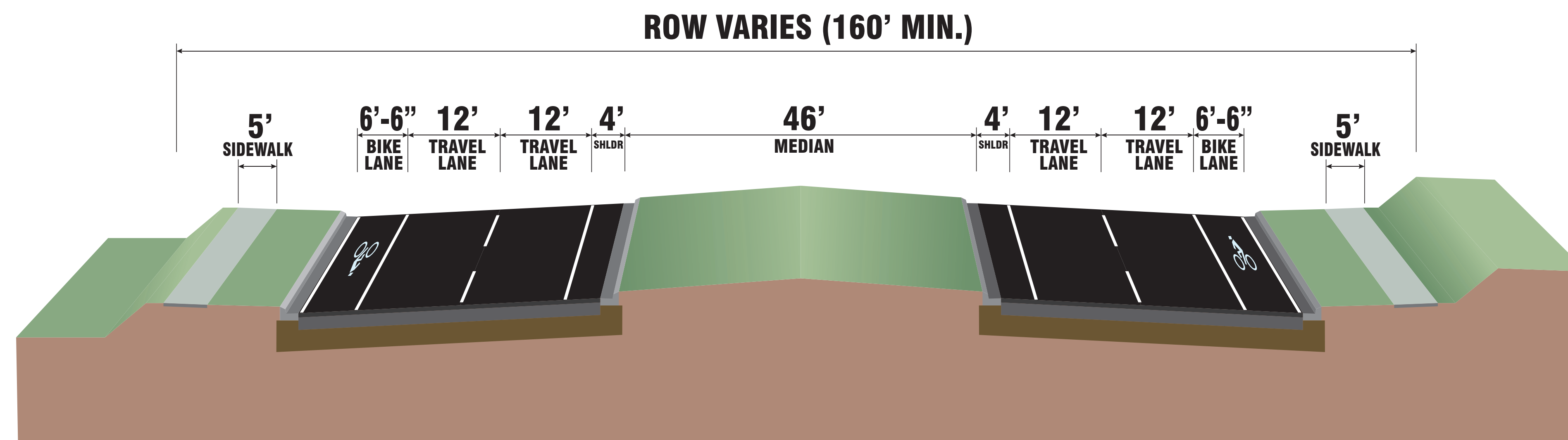
GULF COAST PARKWAY TYPICAL SECTION NEW 4-LANE HIGH-SPEED URBAN
