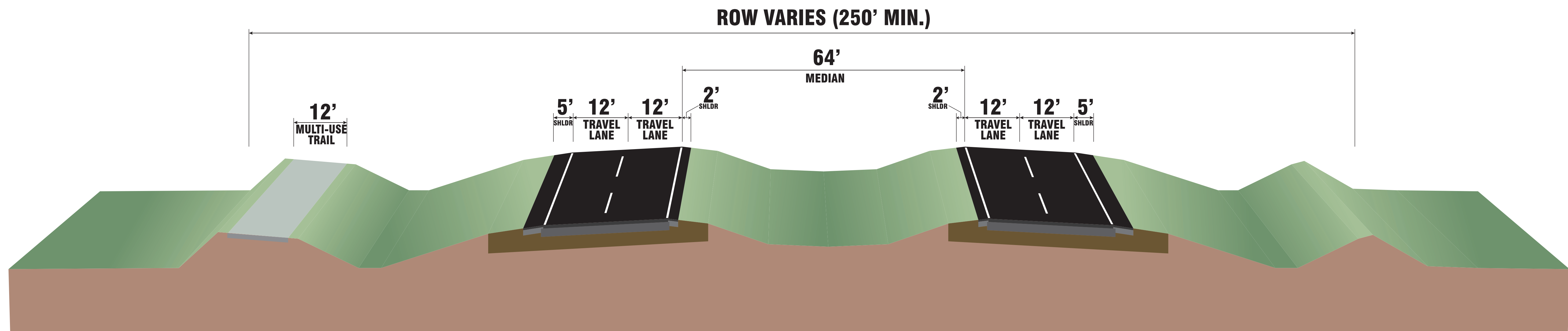
GULF COAST PARKWAY TYPICAL SECTION NEW 4-LANE RURAL
