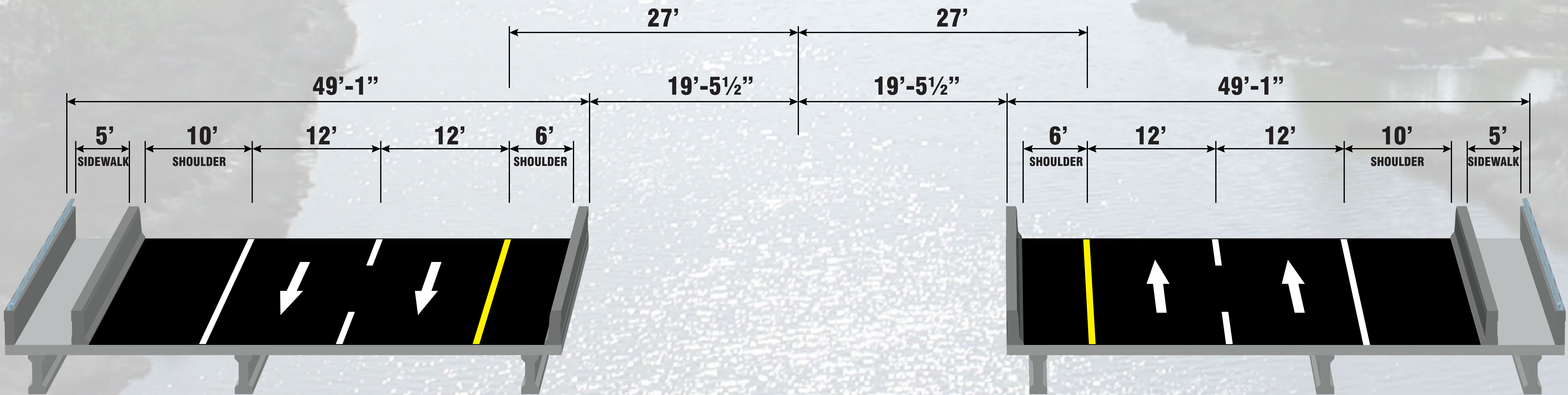
URBAN BRIDGE TYPICAL SECTION DESIGN SPEED 55 MPH
