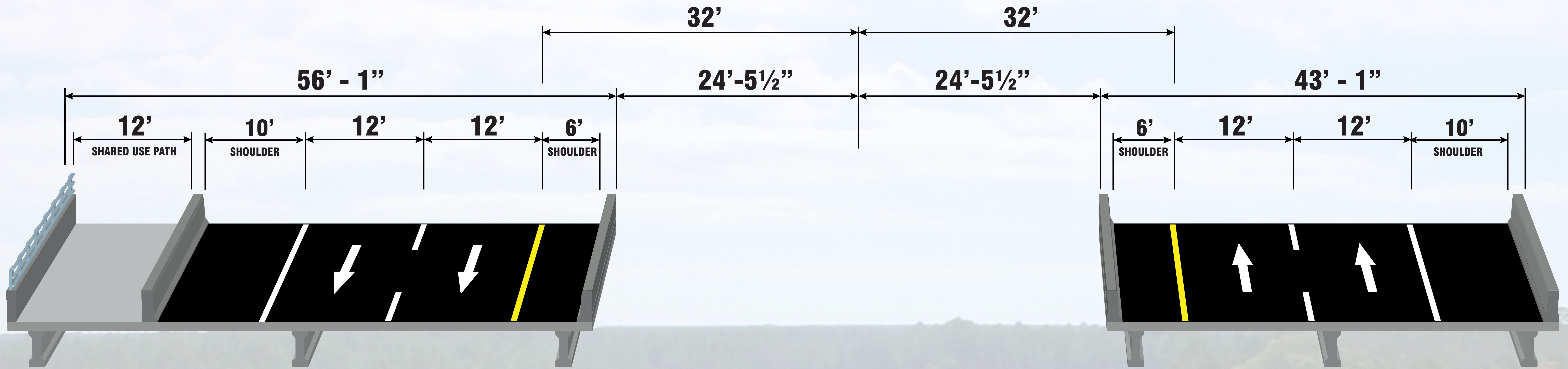
RURAL BRIDGE TYPICAL SECTION DESIGN SPEED 55 MPH
